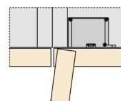
Door opening with stop device at 92°
